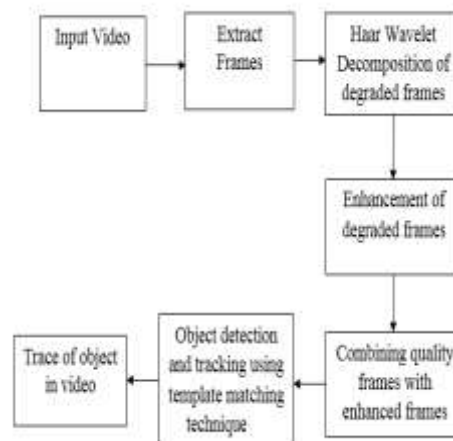
Figure: Architecture of Proposed Method
